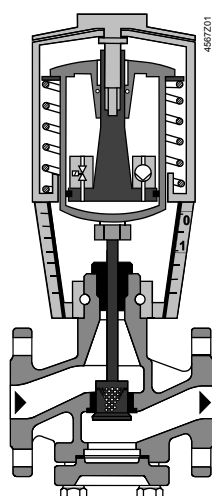
Valve closed
