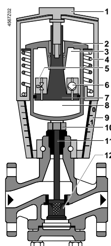
Valve open
